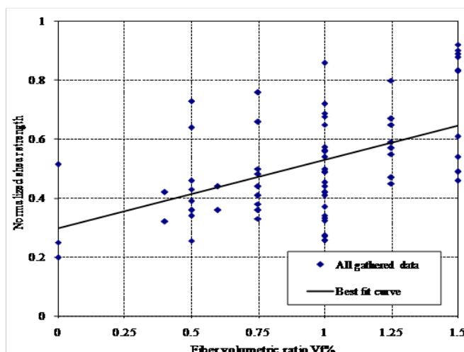
Fig. 9: Relation between fiber volumetric ratio and normalized shear strength of beams
